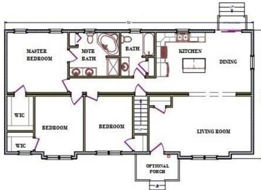
1ST FLOOR
